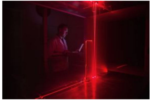
Calibration wind tunnel 2 (PTB)
